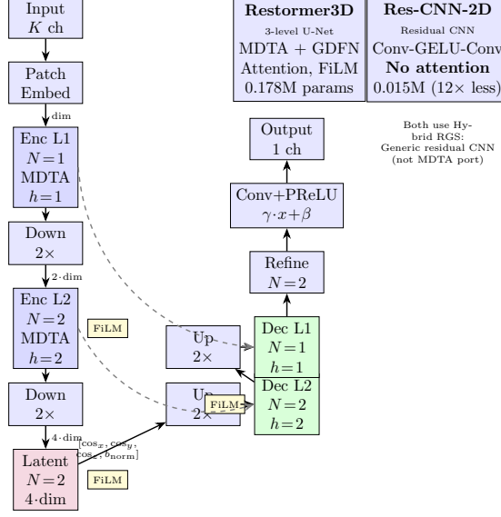
Figure 3: Restormer architecture for Hybrid RGS. (a) Restormer3D internal architecture: A 3-level encoder-decoder with transformer blocks at each stage. The encoder progressively downsamples spatial dimensions ( \times 2 per level) while doubling channel count ( \text{dim} \rightarrow 2 \cdot \text{dim} \rightarrow 4 \cdot \text{dim} , with \text{dim} = 12 ). Each level contains N transformer blocks combining Multi-DConv Head Transposed Self-Attention (MDTA, h heads) and Gated-DConv Feed-Forward Networks (GDFN). The decoder mirrors the encoder with skip connections (dashed gray arrows) and channel-reduction convolutions after concatenation. Refinement blocks and a learned affine output head ( \gamma_{\text{out}} \cdot x + \beta_{\text{out}} ) produce the single-channel denoised volume. Optional FiLM conditioning (yellow boxes) modulates features at three stages using the target gradient’s acquisition metadata [\cos_x, \cos_y, \cos_z, b_{\text{norm}}] ; see Table 6 for evaluation. (b) Volumetric backbone versus lightweight 2D baseline: Restormer3D is a full 3D transformer with hierarchical attention (0.178M parameters). Res-CNN-2D is an independent generic residual CNN with no attention, no hierarchical structure, and 12\times fewer parameters (0.015M), used to test whether the Hybrid RGS objective alone suffices without transformer capacity (Table 4).
