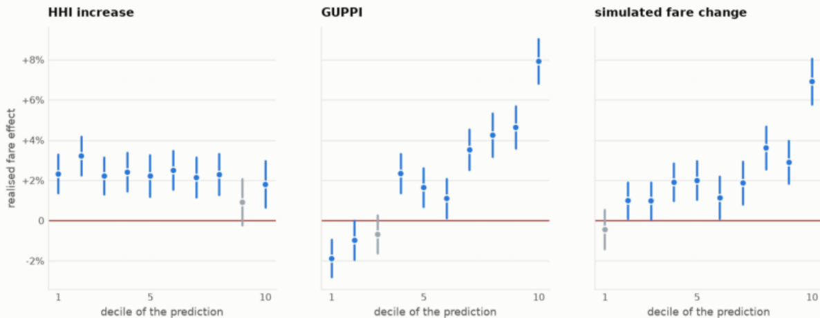
Exhibit 2. Realised effect by decile of each prediction.
