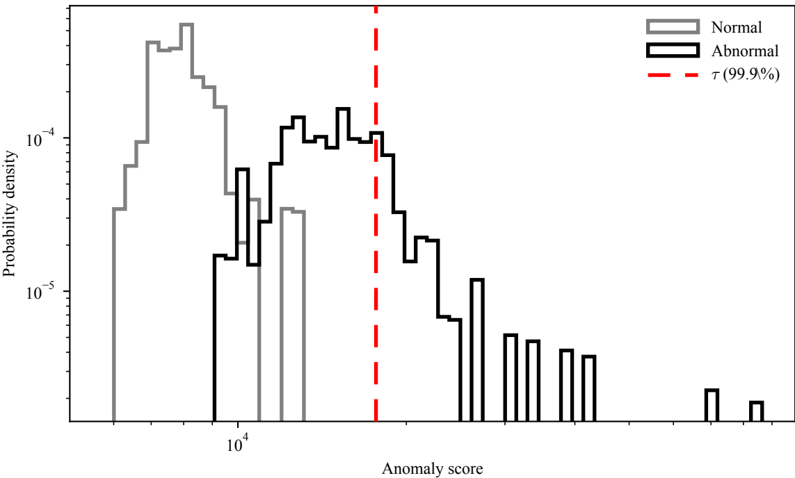
Tail enrichment of morphological anomaly scores
