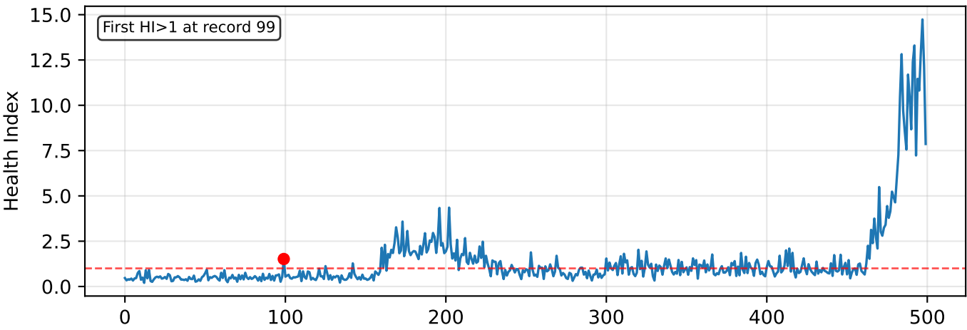
IMS 2nd test
