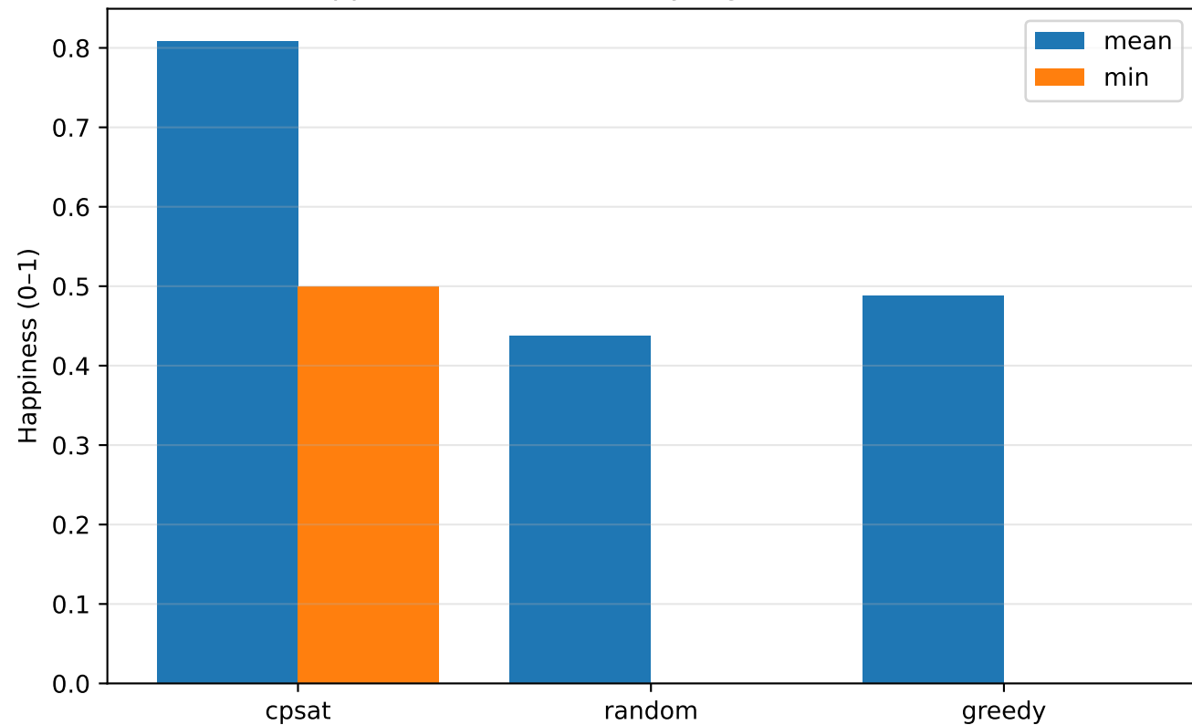
Happiness mean vs min by algorithm (utilitarian)
