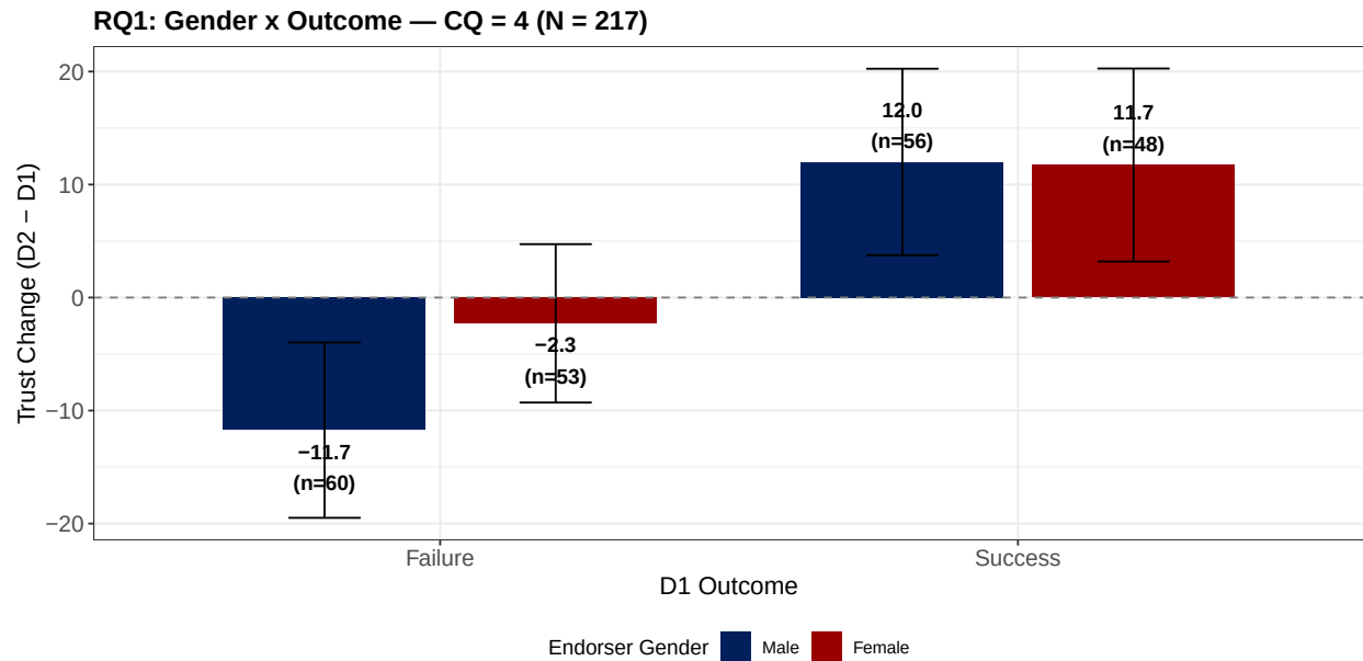
Figure 2: RQ1: CQ = 4
