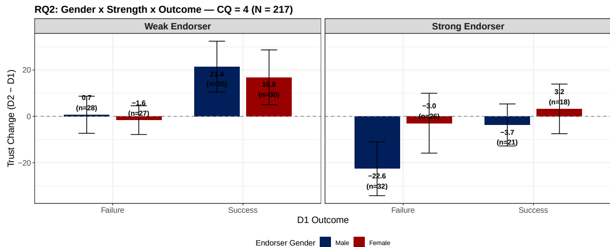
Figure 5: RQ2: CQ = 4
