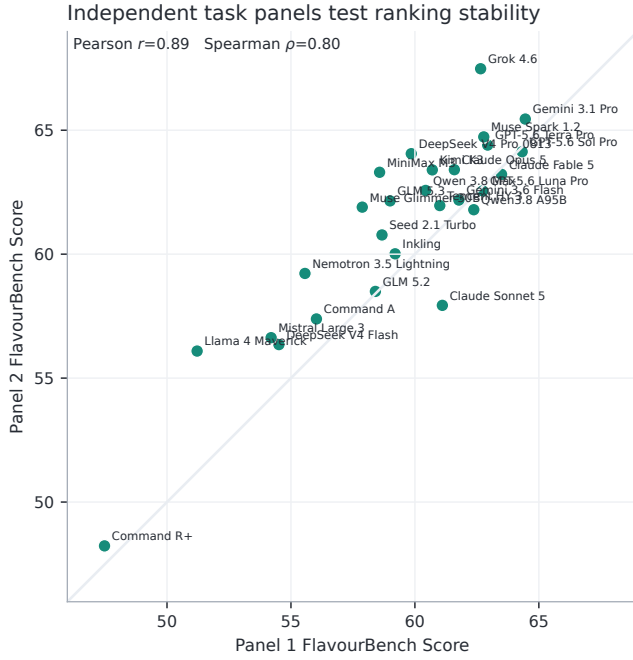
Figure 3: Panel-1 versus panel-2 FlavourBench Score for every endpoint. The diagonal marks exact agreement. Each point aggregates 89 tasks per family; the joint analysis uses 534 unique anchor clusters.
