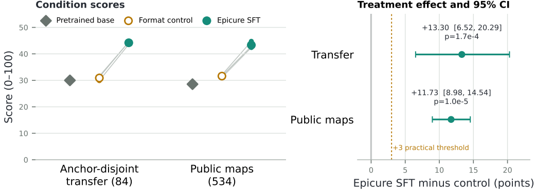
Figure 6: Held-out scores and matched treatment effects. Small points are training seeds; connecting lines pair the control and treatment initialized with the same seed. The right panel reports the prespecified crossed-bootstrap interval. The dashed line marks the three-point practical threshold, not a null hypothesis.
