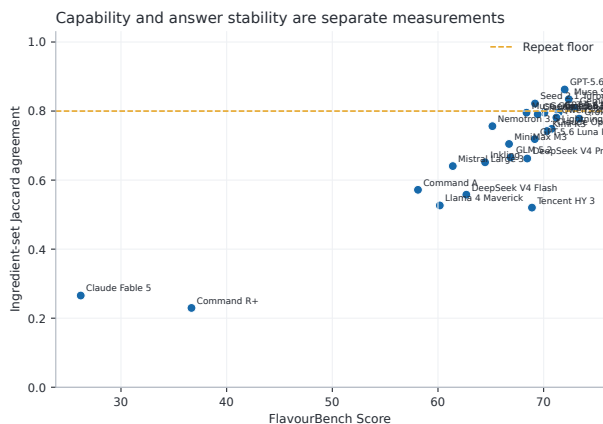
Figure 5: Primary score versus ingredient-set agreement under label permutation. The dashed line is the pre-registered 0.80 repeatability requirement for a definitive top-model claim.
