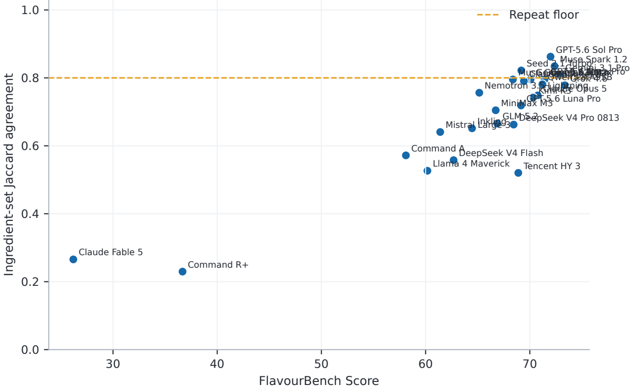
Capability and answer stability are separate measurements
