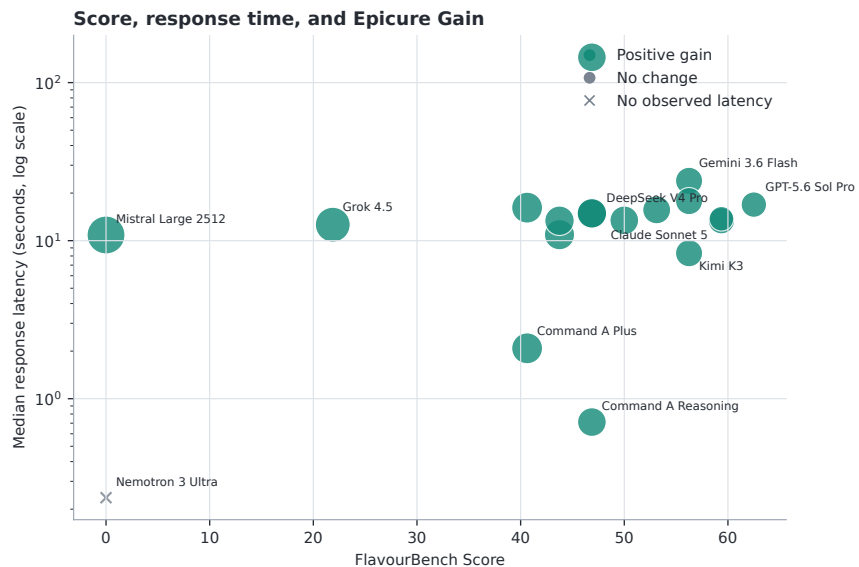
Figure 6: FlavourBench Score, response time, and Epicure Gain. Response time uses a log scale. Point size increases with the magnitude of gain; colour indicates its direction. An × marks a route with no observed response time.
