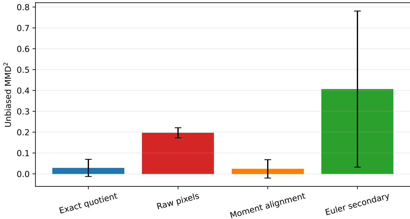
RxRx1 quotient discrepancy across acquisition-transform seeds
