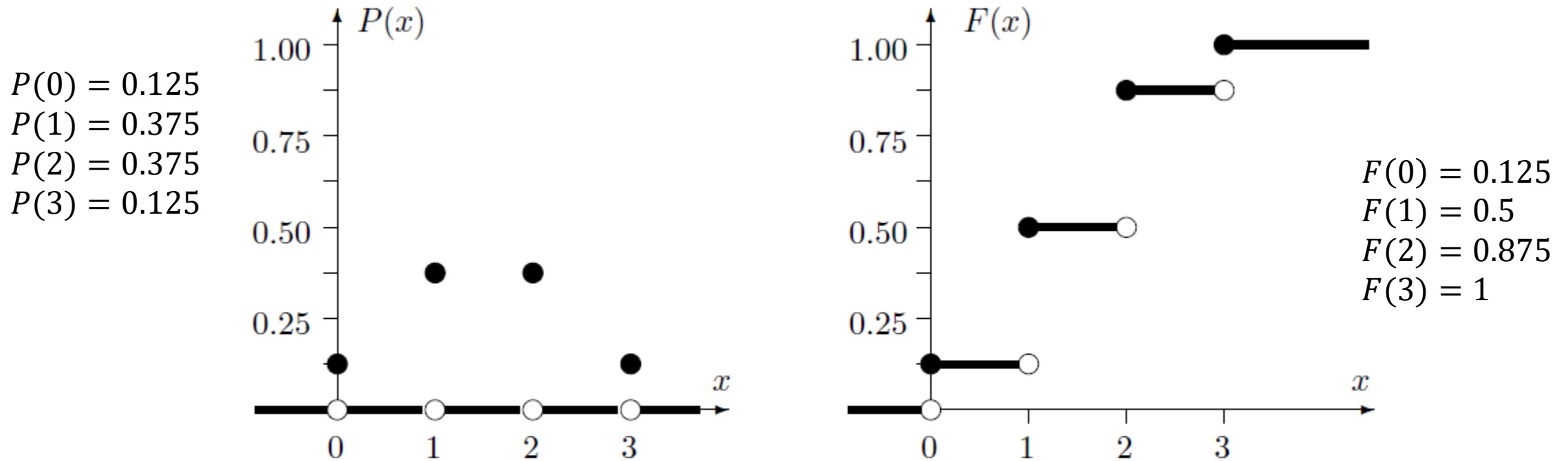
FIGURE 3.1: The probability mass function P(x) and the cumulative distribution function F(x) for Example 3.1. White circles denote excluded points.
