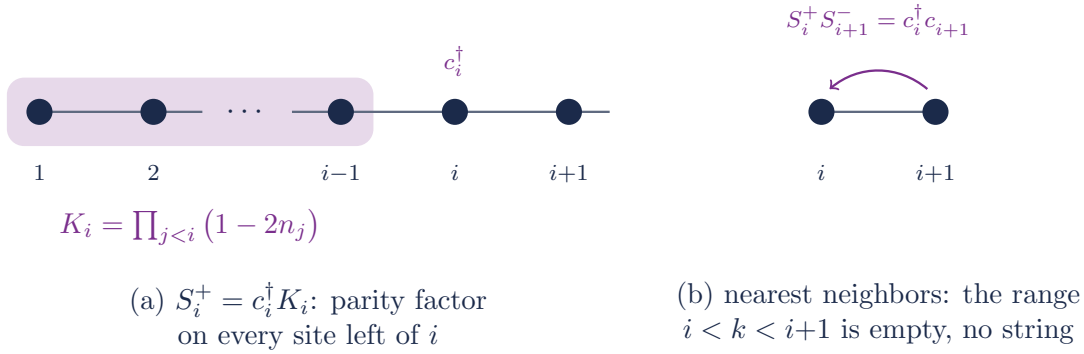
Figure 12: The Jordan-Wigner string, and why it usually vanishes from sight. (a) The dictionary of Eq. (70) attaches to c_i^\dagger the parity factor K_i = \prod_{j < i} (1 - 2n_j) , one factor for every site to the left of i , shaded here. That trailing string is what repairs the mismatch between anticommuting fermions and commuting spins. (b) On a nearest-neighbor bond the product in Eq. (71) runs over the empty range i < k < i + 1 , so the string collapses to 1 and the spin bilinear reduces to the bare hopping. This is why the models we build matrix product state Hamiltonians for never meet the string explicitly.
