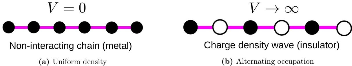
Figure 7: The two solvable limits of Eq. (38), with filled circles marking occupied sites and open circles empty ones. (a) At V = 0 the chain is a free tight-binding metal at half filling, with the same average density on every site and a unique ground state. (b) As V \rightarrow \infty the hopping becomes irrelevant and the interaction alone selects the alternating 1, 0, 1, 0, \dots pattern. Shifting that pattern by one site produces a second state of identical energy, and this twofold degeneracy is the defining signature of the charge-density wave.
