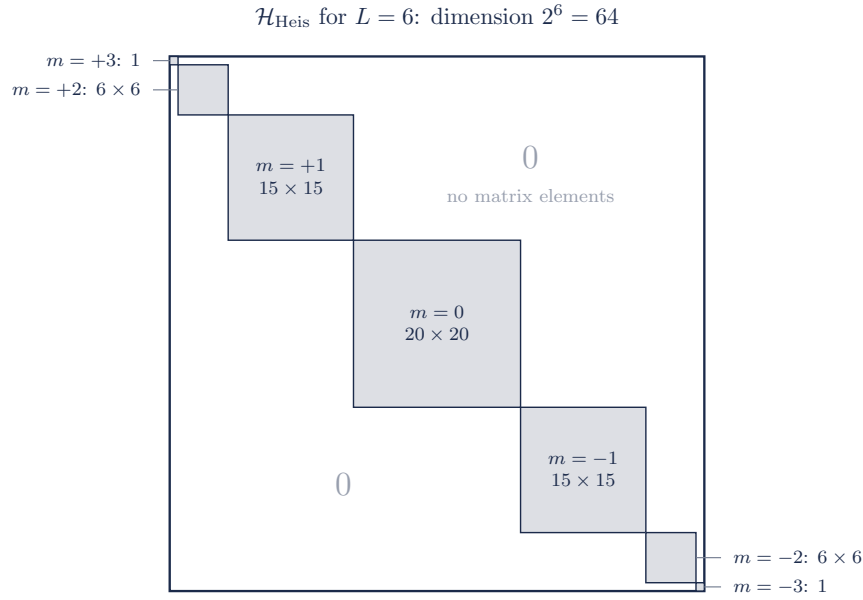
Figure 5: Block structure of \mathcal{H}_{\text{Heis}} in the S_{\text{tot}}^z basis, drawn for L = 6 with the blocks to scale. Because S_{\text{tot}}^z is conserved, the Hamiltonian never connects basis states with different numbers of up spins, so the 2^L \times 2^L matrix falls apart into one block per magnetization sector, of dimension \binom{L}{L/2+m} as in Eq. (28), with nothing at all outside them. Each block is diagonalized completely independently of the others, and even the largest one, at m = 0 , is already smaller than the full space by a factor \sim \sqrt{L} .
