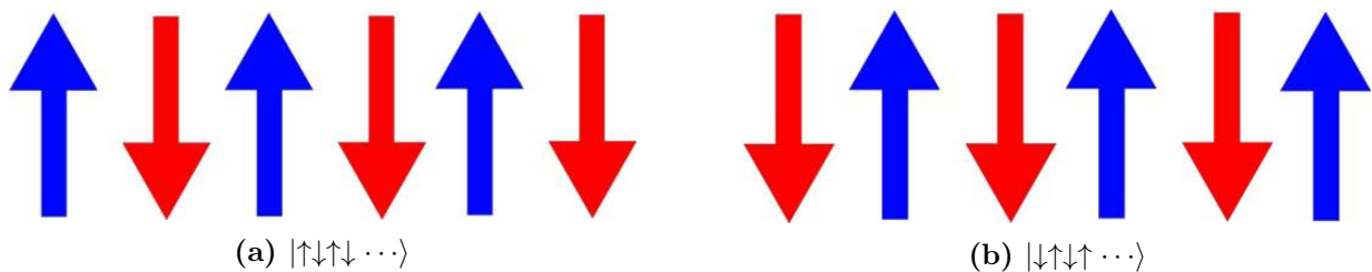
Figure 4: The two classical ground states of Eq. (25) at the Ising endpoint J_{xy} = 0 . Each is a product state with a definite S^z on every site, each carries a finite staggered moment, and the two are exchanged by time reversal. In the thermodynamic limit they are exactly degenerate and the system picks one of them, which is what symmetry breaking means here. On a finite chain they are instead split by a tiny amount, and watching that splitting grow as J_{xy} \rightarrow 1 is how the crossover to the unique, entangled Heisenberg ground state shows up in the spectrum.
