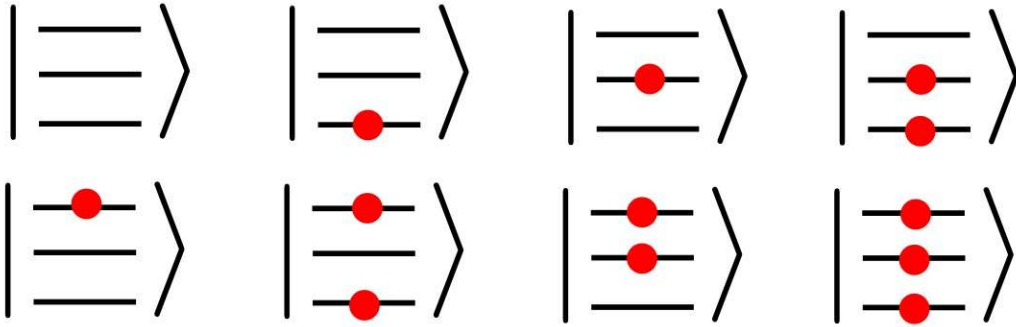
Figure 6: The complete many-body basis of three spinless orbitals, drawn as three levels per state with a dot on every occupied one. Reading across, there is one empty configuration, three with a single electron, three with two electrons and one completely filled state, for 1 + 3 + 3 + 1 = 8 = 2^3 basis states in total. Every additional orbital doubles this count, because each orbital is independently either empty or filled, and that doubling is exactly the exponential wall that separates many-body from single-particle physics.
