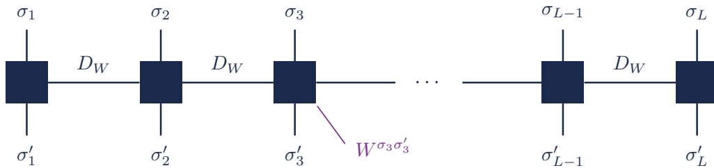
Figure 14: A matrix product operator, the operator counterpart of the matrix product state we used throughout Session 4. Each site tensor W^{\sigma_i \sigma'_i} carries two physical legs, one for the row index \sigma_i and one for the column index \sigma'_i , on top of the same two internal bond legs as before, here of dimension D_W . For a nearest-neighbor Hamiltonian those internal bonds only need to carry a handful of states, which is enough to encode \mathcal{H} exactly rather than approximately.
