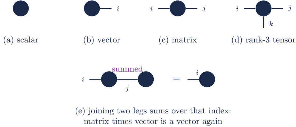
Figure 13: Diagrammatic notation for tensors: a dot with one leg per index. (a) A scalar has no legs, (b) a vector has one, (c) a matrix has two, and (d) a rank-three tensor has three. (e) Summing over an index shared by two tensors is drawn by joining the corresponding legs into a single line, so a two-legged dot joined to a one-legged dot leaves one free leg and is therefore a vector again, exactly as matrix-vector multiplication should be.
