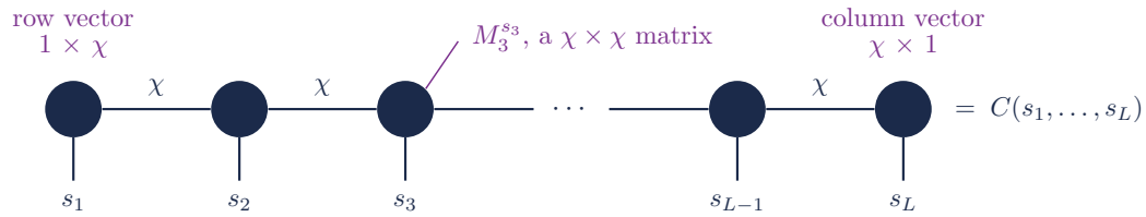
Figure 8: The matrix product state of Eq. (52) drawn as a tensor network. Each site carries one tensor M_n^{s_n} , with a vertical physical leg running over the d local states of that site and horizontal bond legs of dimension \chi joining it to its neighbors. Joining two legs means summing over the shared index, so contracting the horizontal legs from left to right is precisely the matrix product of Eq. (52). The two end tensors carry a single bond leg each, a row vector and a column vector, which is why the whole contraction collapses to one number.
