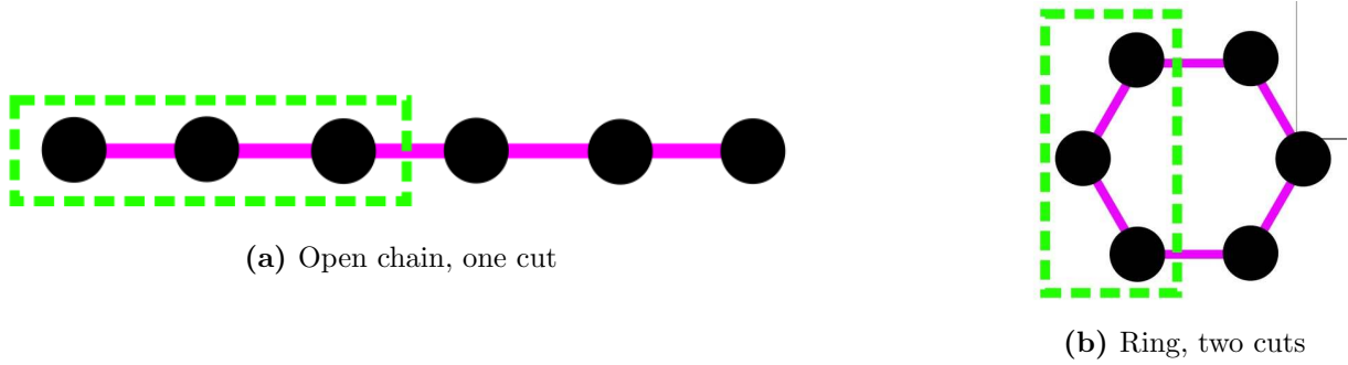
Figure 10: Why open boundaries are so much cheaper. The dashed line marks the block A whose entanglement entropy we compute. (a) On an open chain, a contiguous block borders the rest of the system at a single point, so one bond is severed. (b) On a ring the same block is adjacent to the rest at both of its ends, so any bipartition severs two bonds and each one contributes, roughly doubling S_A . Through the bound of Eq. (62), a doubled entropy costs us the square of the bond dimension for the same accuracy.
