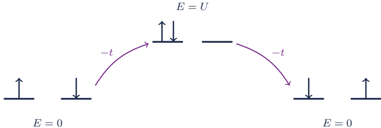
(b) antiparallel spins: virtual double occupancy at energy U , second order gives E_{\text{singlet}} \approx -4t^2/U
