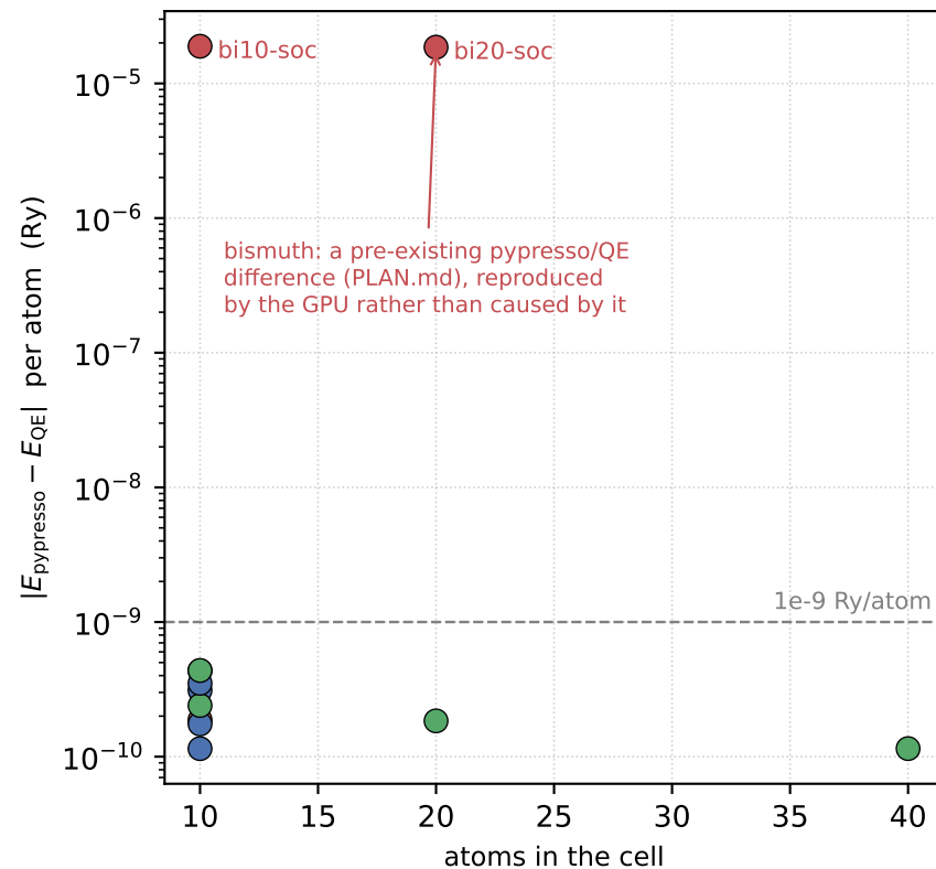
Agreement with Quantum ESPRESSO
