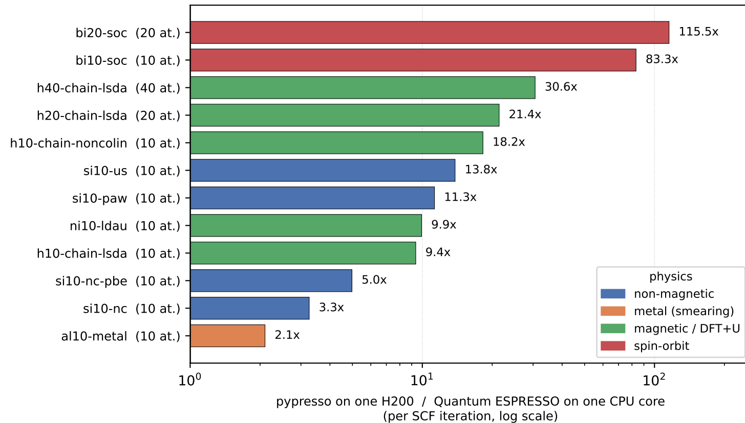
Speedup per SCF iteration
