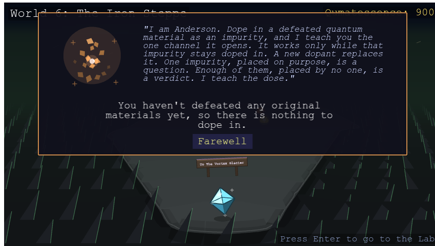
Figure 2: Anderson's impurity-doping panel
