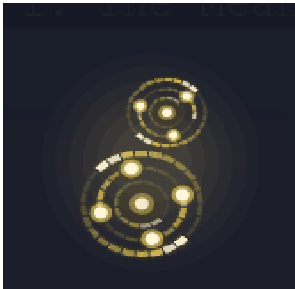
Figure 20: Noether: two circling cells of golden current, motes carried round and round and never lost
