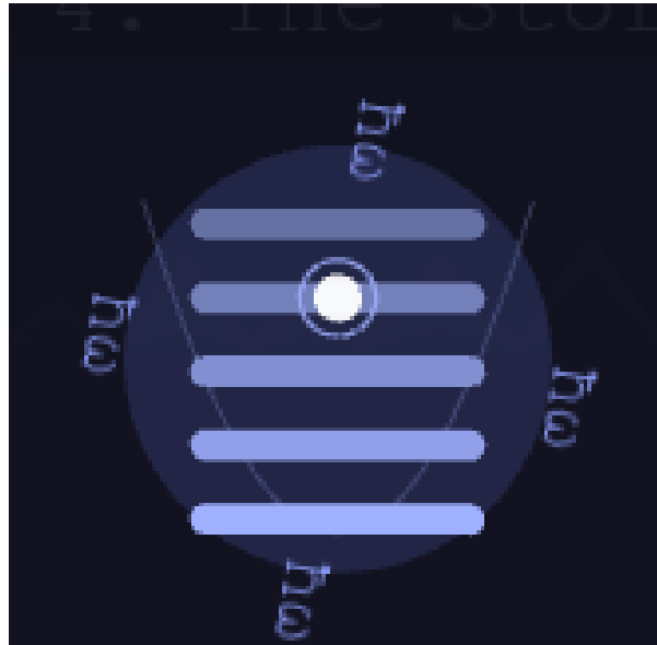
Figure 26: Landau: a ladder of flat, evenly spaced levels with one electron jumping between them, drawn over the faint parabola of the band they came from
