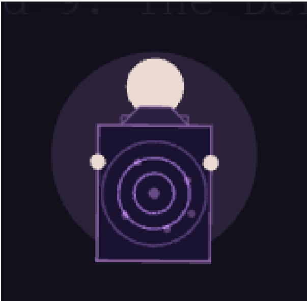
Figure 36: Franklin: a figure holding up a sheet of film carrying diffraction rings and their scattered spots
