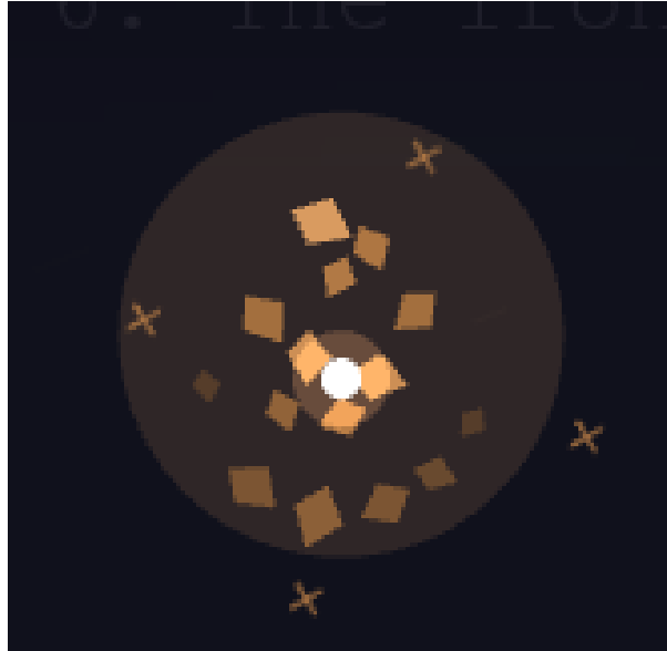
Figure 30: Anderson: a scatter of disconnected fragments with no outline at all, drifting around one bright localized core
