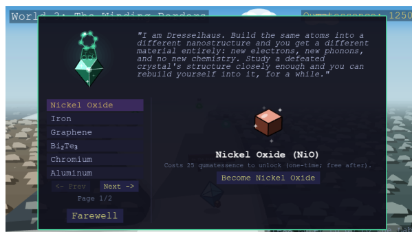
Figure 26: Dresselhaus's panel: crystals available to become, the selected one drawn beside its 25-qumatessence cost
