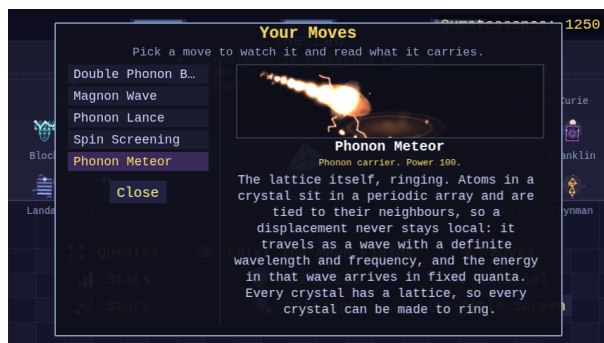
Figure 17: The Lab's Moves station, an Ultimate meteor playing on its stage beside what the move carries and what a phonon is
