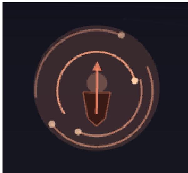
Figure 35: Kondo: a small local moment drawn as an arrow, sitting inside two counter-rotating screening shells
