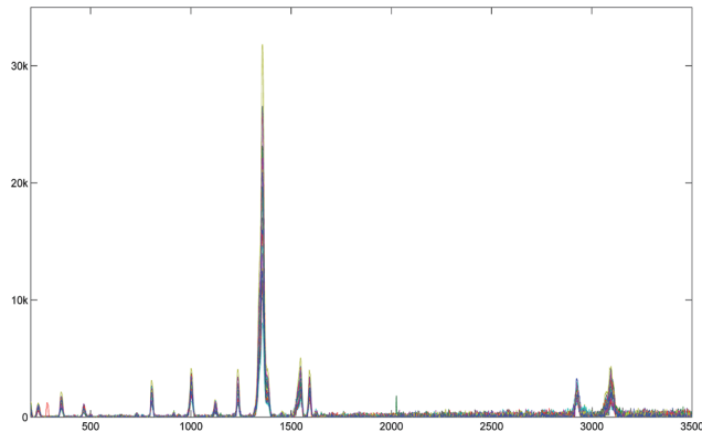
Fig. 12 Baseline corrected 26DNT Raman spectra.
