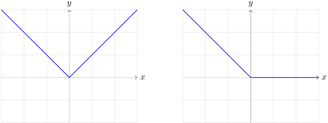
Figure 2: Example and counterexample of condition (C3)
