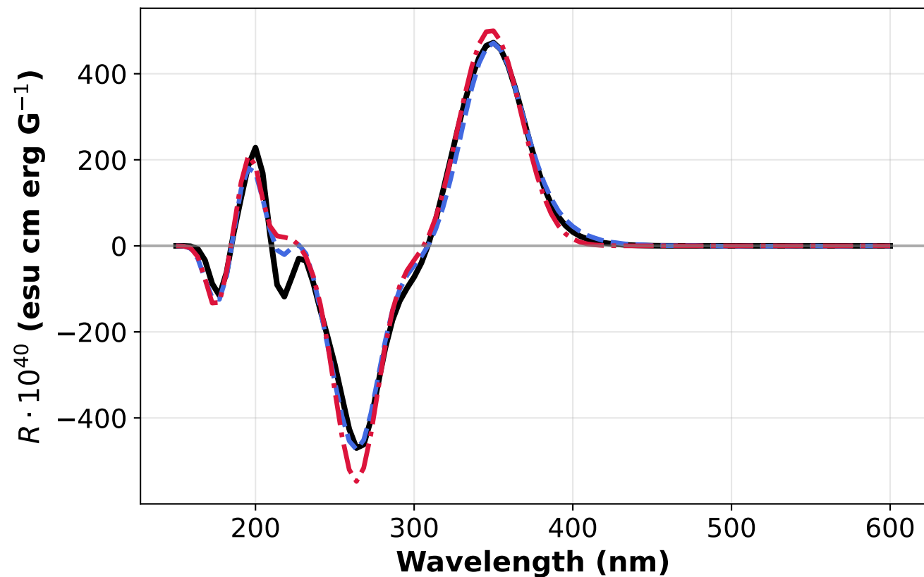
6Heliceno_4-COOH MAE (E2E/PINN): 12.8 / 17.5 | Cos: 0.992 / 0.987
