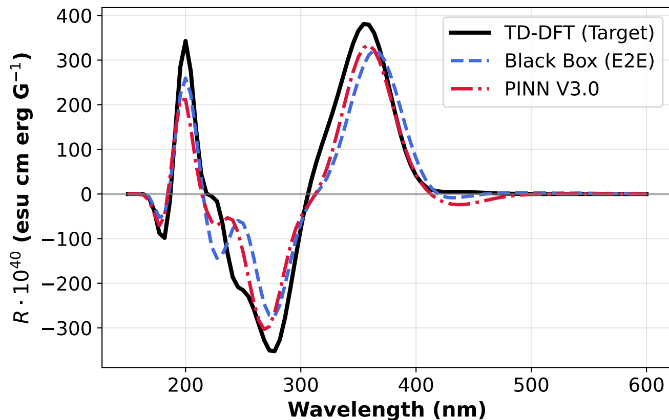
6Heliceno_5-CN_8-CC_9-OMe_11-CN MAE (E2E/PINN): 21.5 / 22.0 | Cos: 0.977 / 0.968
