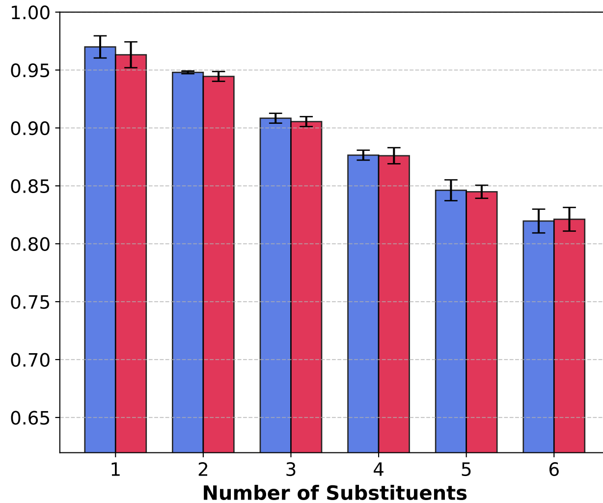
R 2 Score ↑
