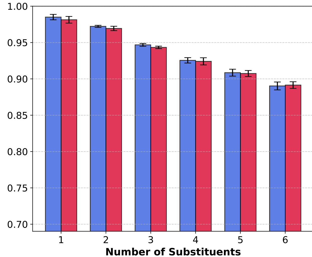
Cosine Similarity ↑
