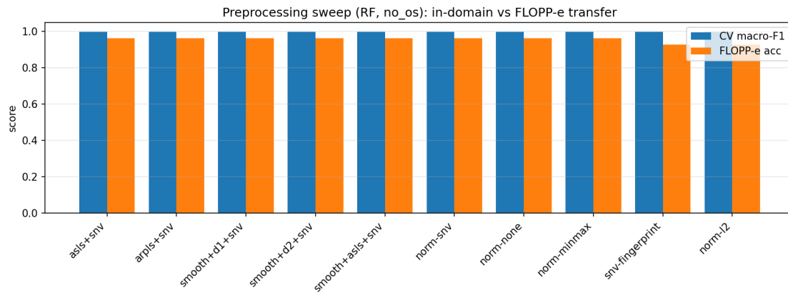
Figure 2: Preprocessing sweep (RF, c4+c8). Every config sits at ceiling in-domain.
