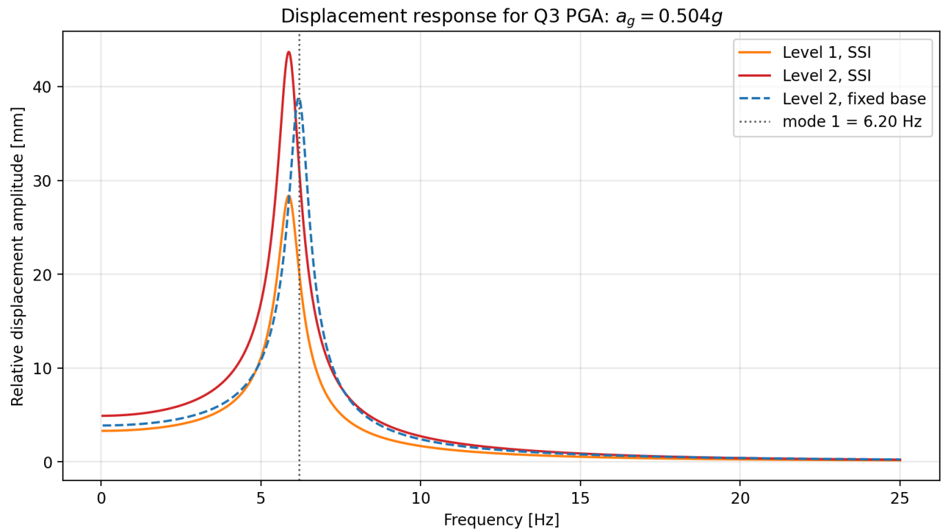
Figure 3. Displacement response at the two levels for a_g = 0.504g .
