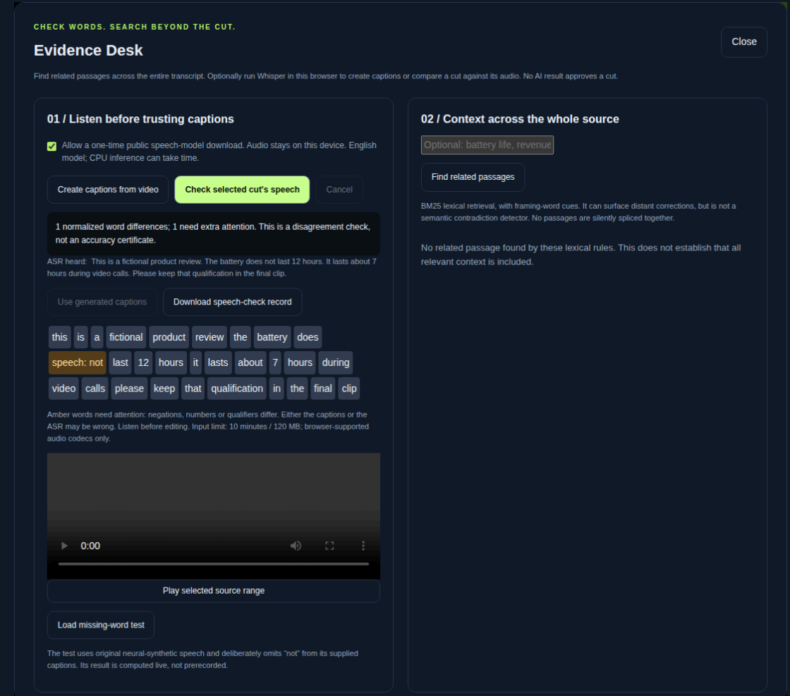
Actual browser inference on the fictional missing-word fixture.
