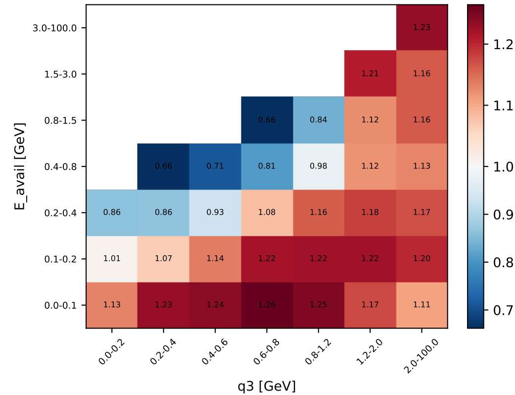
MINERvA ME FHC, 1.06 \times 10^{21} POT
