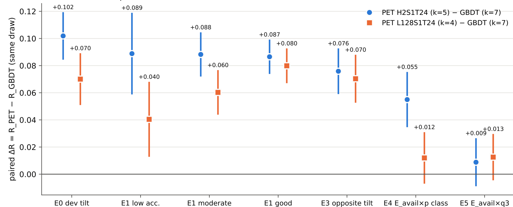
Paired differences per FB draw, mean \pm 95% t interval
