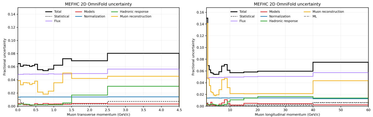
Figure 11: Fractional uncertainty on the 2D cross section projected onto p_T (left) and p_{||} (right), grouped by source in the style of Figs. 6–7 of Ref. [1]: flux, interaction models, normalisation, hadronic response, muon reconstruction, and the statistical band.
