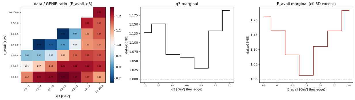
Figure 12: Data/GENIE-CV ratio of the 4D unfold projected onto the (E_{\text{avail}}, q_3) plane (left; blank cells are kinematically empty), with the q_3 (centre) and E_{\text{avail}} (right) marginals. The E_{\text{avail}} marginal reproduces the 3D low-recoil excess; the joint plane shows the data – MC discrepancy to carry genuine q_3 structure (the ratio rising with q_3 across the quasielastic- \Delta dip). GENIE central value, no 2p2h in the base event-generator list.
