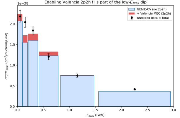
Figure 11: Re-generating GENIE with the empirical Valencia 2p2h enabled (red, stacked on the no-2p2h CV) fills part of the low- E_{\text{avail}} dip — about half the data-CV gap, the remainder being the MINERvA-tune enhancement.
