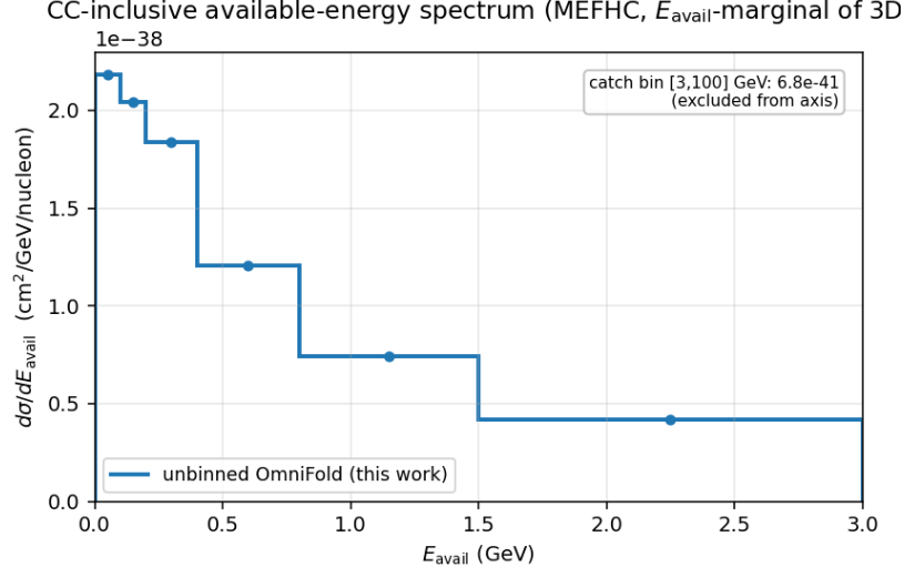
Figure 7: Unfolded available-energy spectrum d\sigma/dE_{\text{avail}} , the 1D projection of the 3D measurement. The wide [3, 100] GeV catch bin (value annotated) is excluded from the axis.
