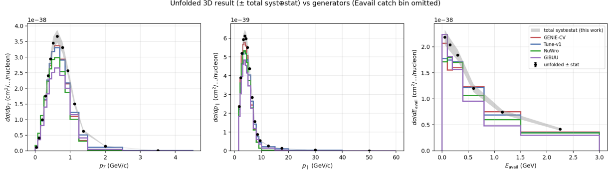
Figure 9: 1D projections of the unfolded 3D cross section (black, with the combined-covariance systematic band) versus four generator predictions produced at truth level: GENIE 2.12 CV, MINERvA Tune v1, NuWro 21.09, and GiBUU 2019. On p_T and p_{||} the models track the data shape; on E_{\text{avail}} they split, and all under-predict the data at low available energy. The wide E_{\text{avail}} catch bin is omitted from the axis.
