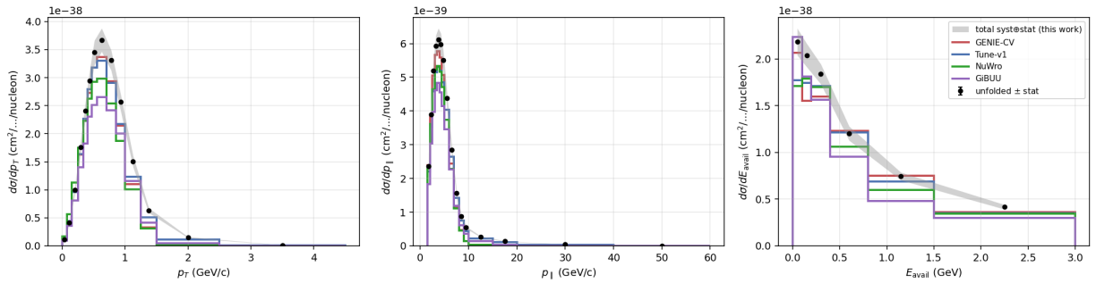
Unfolded 3D result ( \pm total syst+stat) vs generators (Eavail catch bin omitted)
