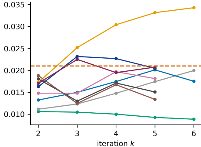
neutrons \times 1.3 : E_{\text{avail}} residual L1
