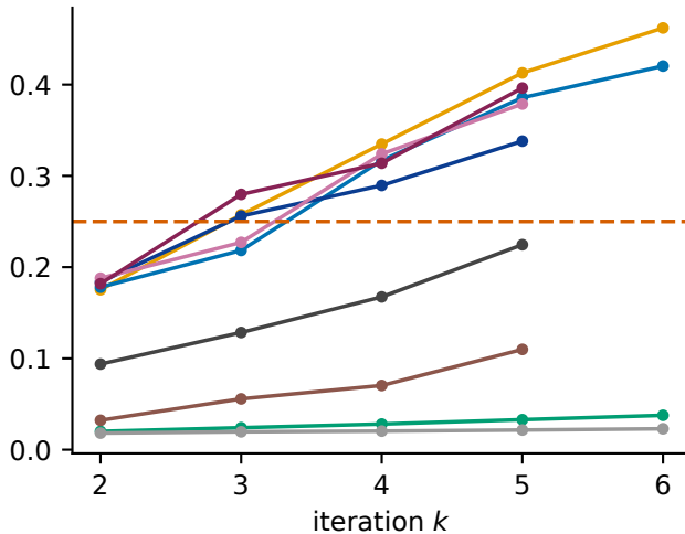
protons \times 1.3 : joint E \times p recovery
