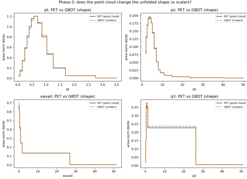
Figure 5: Method cross-check: the point-cloud PET unfold (solid) versus the scalar GBDT unfold (dashed), area-normalised 1D projections on each axis. The two agree to 2 % to 4 % median per bin, confirming the unbinned technique is robust to the classifier family and scales from tabular features to permutation-invariant point clouds. PET here is a 2M-event, 2-iteration run (a method demonstration, not a separate physics result).
