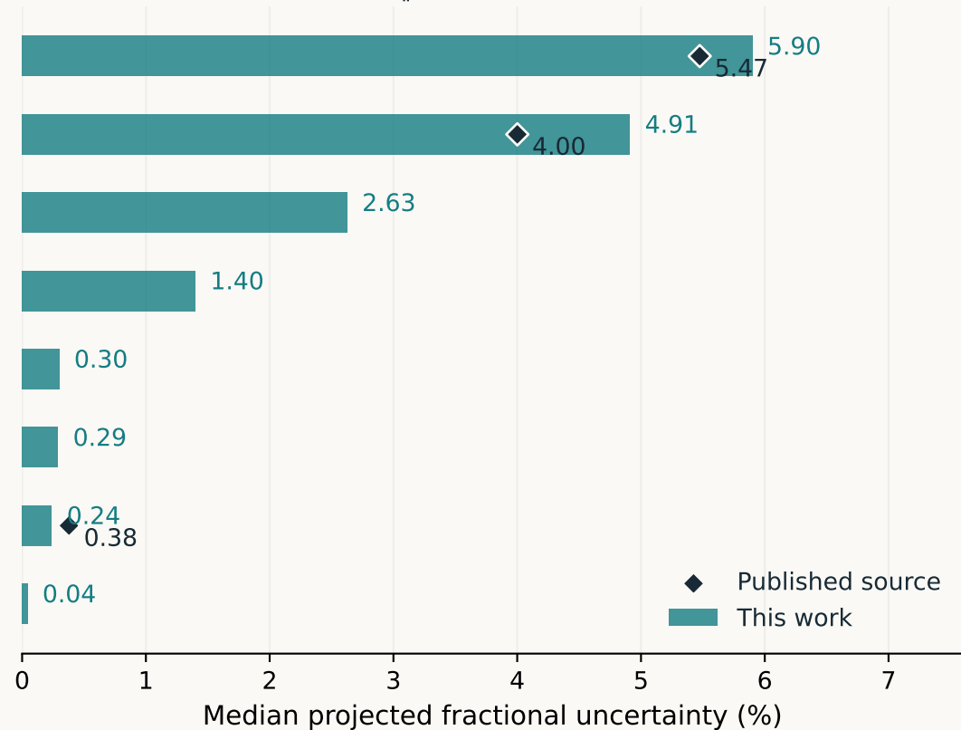
p_{\parallel} projection
