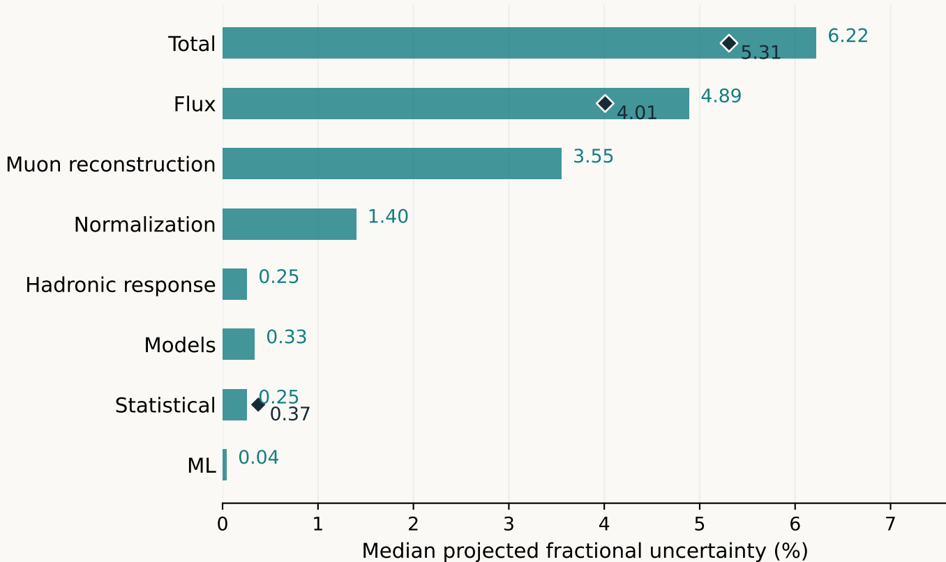
p_T projection
