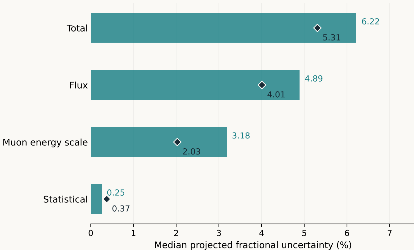
p_T projection
