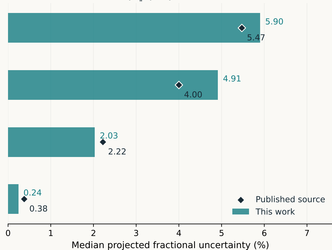
p_{\parallel} projection
