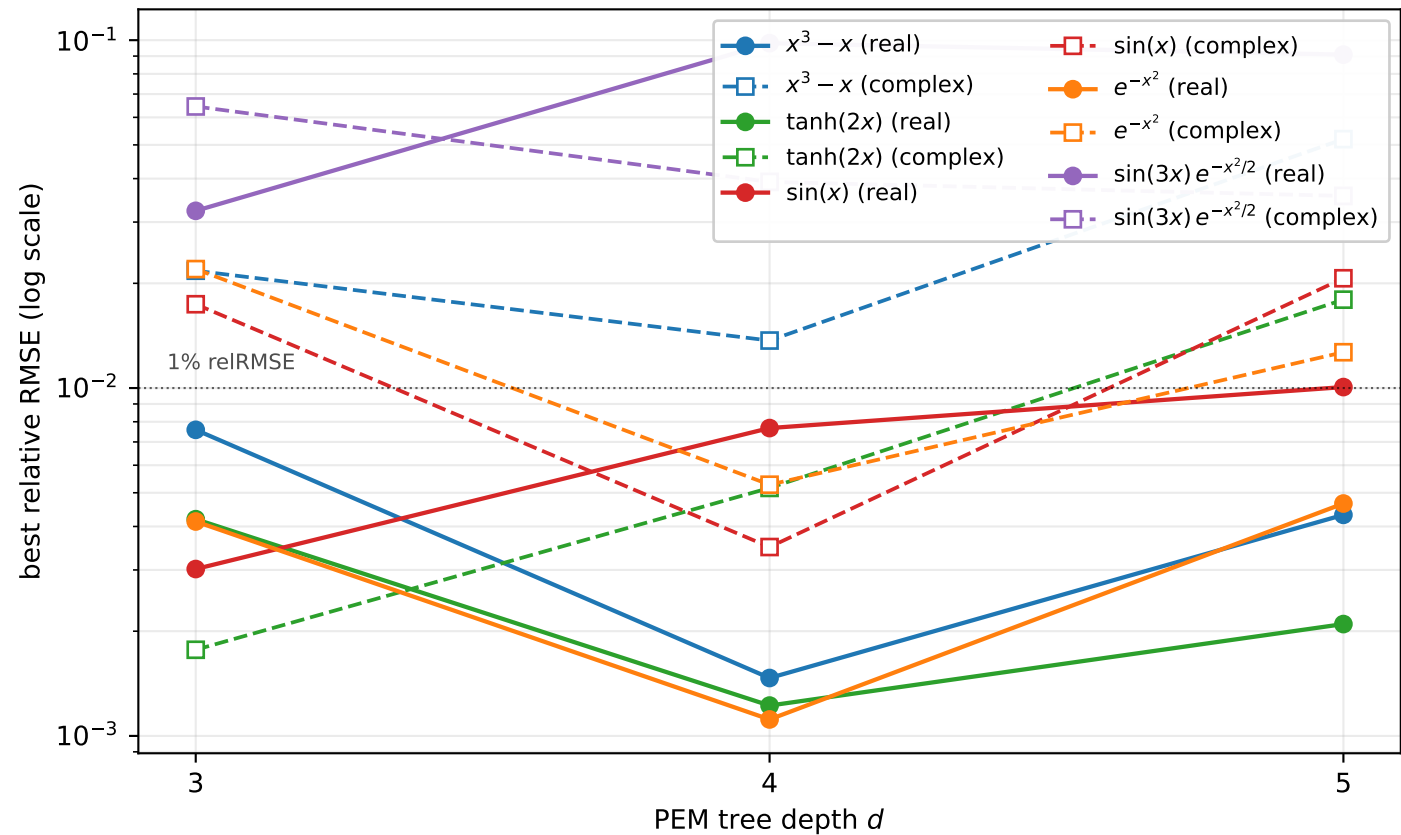
Practical universality of PEM trees: best relRMSE vs depth Adam multi-restart + LBFGS, 30 s/cell, single CPU
