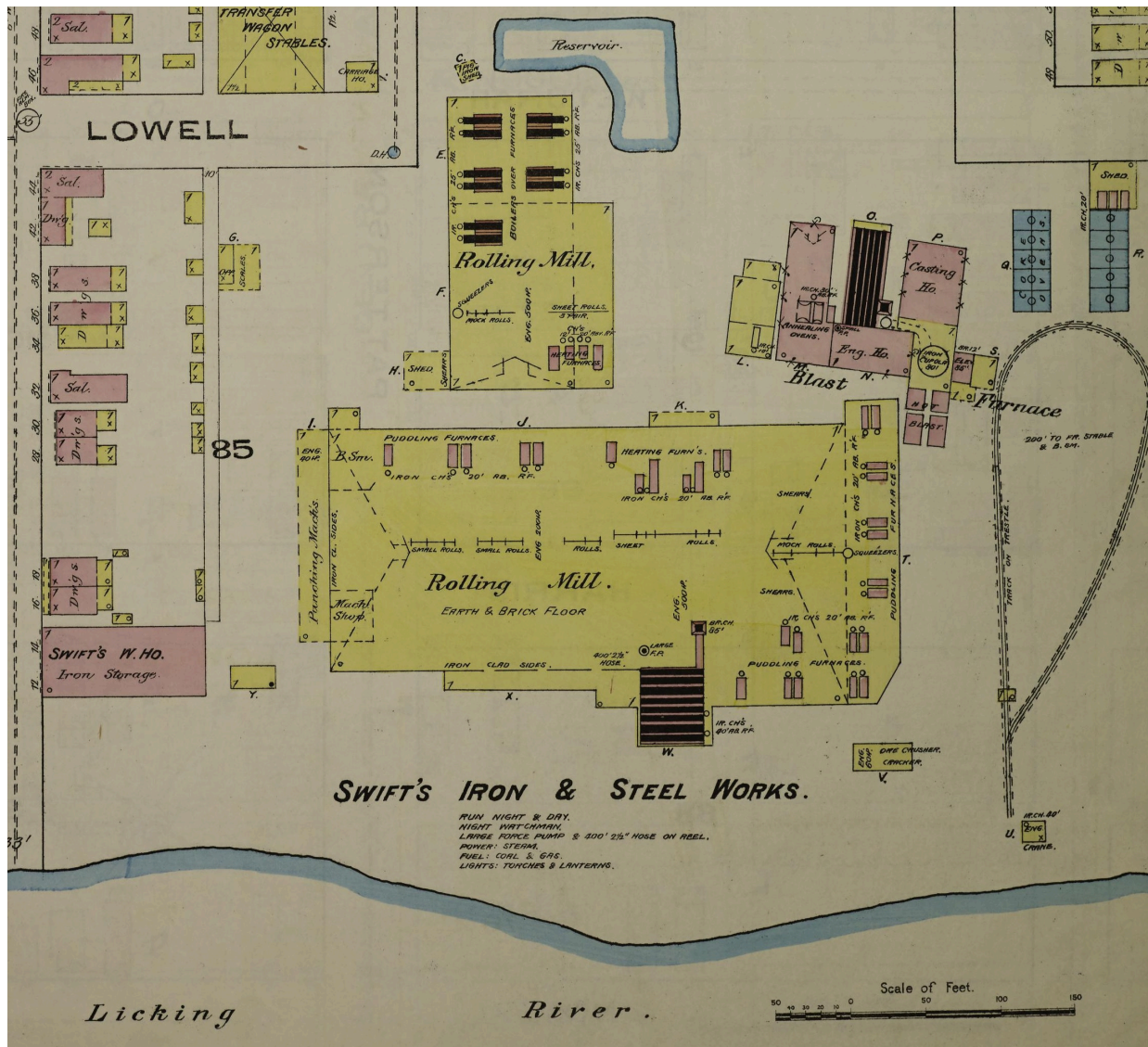
Figure 12: Swift's Iron & Steel Works beside the Licking River in 1886. The sheet labels rolling mills, puddling furnaces, heating furnaces, rolls, shears, boilers, and a blast furnace. August Burkart worked as a rolling-mill catcher, although no surviving record yet identifies this as his employer. Library of Congress, Geography and Map Division, Sanborn Maps Collection; public domain. Open sheet 11.
