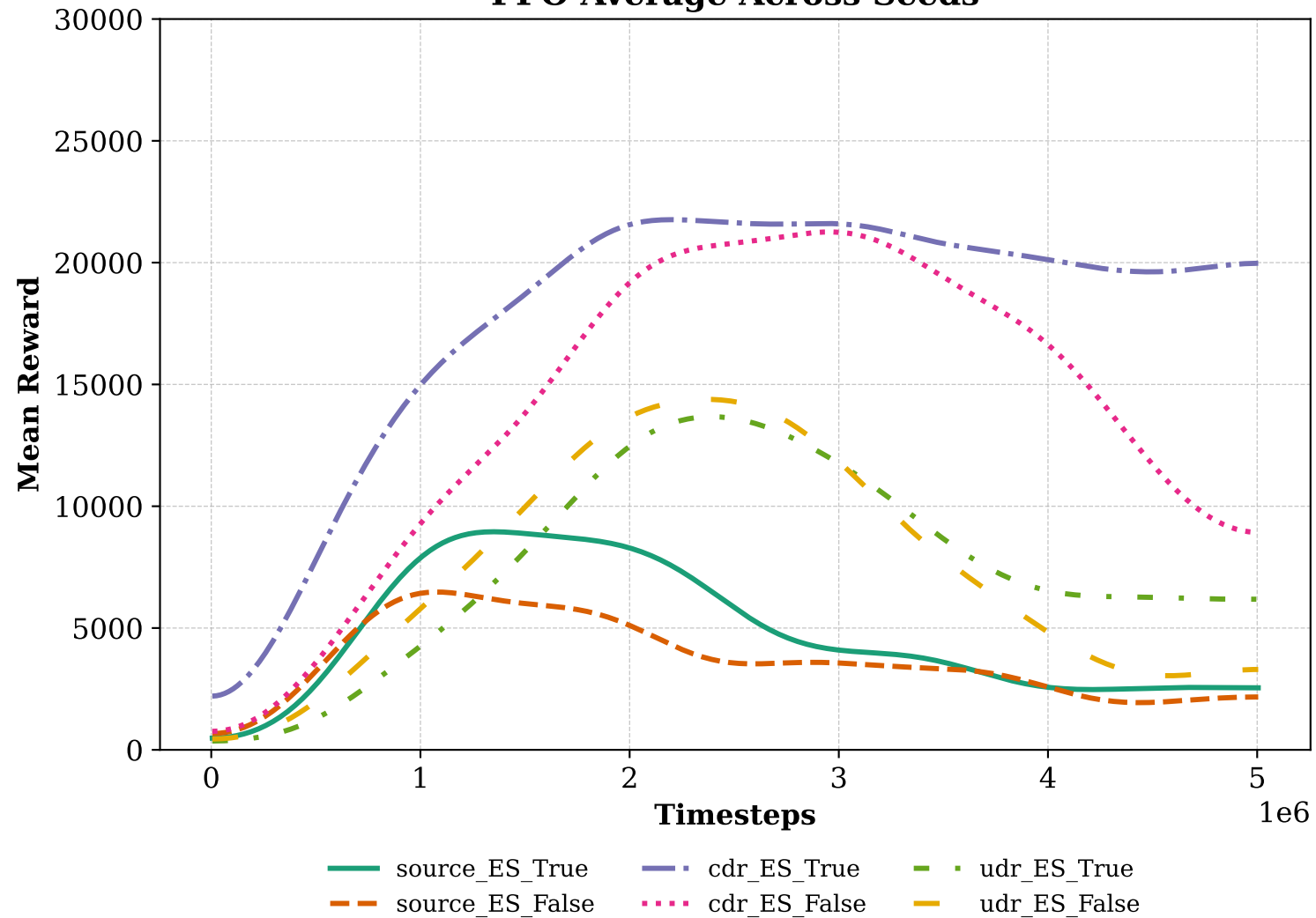
PPO Average Across Seeds
