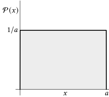
Figure 9.2: The classical probability density for the infinite square well. The shaded area must be equal to one – we must be able to find the particle in the box with 100% probability.
