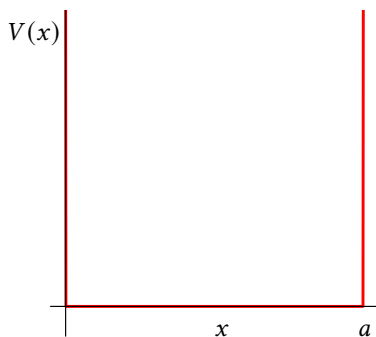
Figure 9.1: The potential energy for the infinite square well.
