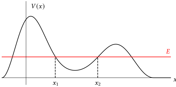
Figure 8.3: A generic example of a potential energy. For a particle of total energy E , the turning points are at x_1 and x_2 .
