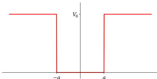
Figure 8.1: The potential energy of the finite square well.
