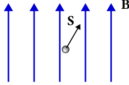
Figure 7.1: An electron in a magnetic field.
