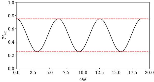
Figure 7.2: The probability \mathcal{P}_{+x} of measuring the electron to have S_x = \hbar/2 as the state evolves in time. The parameter \theta = \pi/6 in this case.
