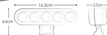
LUZ LED DUAL
