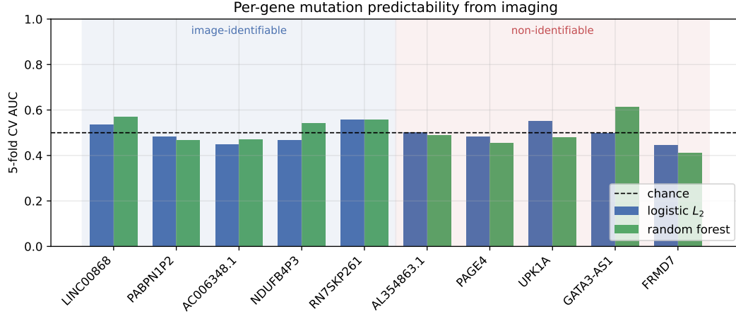
Figure 11: Per-gene mutation predictability on TCGA-KIRC. Five high-recoverability and five low-recoverability mutated genes, two classifiers, 5-fold CV. All bars sit within sampling noise of the chance line at 0.5.
