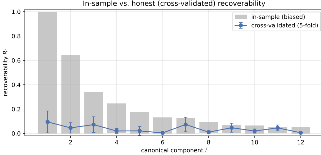
Figure 8: Recoverability spectrum on TCGA-KIRC. In-sample \hat{R}_i (grey) tracks the high-dimensional bulk; cross-validated \hat{R}_i (blue, 5-fold) collapses to a flat residual near zero. The gap is the overfitting predicted in Section 10.5, regime 2–3. Contrast with the synthetic instance of Fig. 5, where CV tracks the planted truth.
