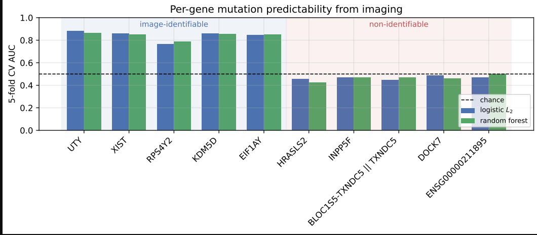
Figure 19: Per-gene predictability on ADNI. Five high- and five low-recoverability transcripts, two classifiers, 5-fold CV. The high-recoverability group reaches AUC \approx 0.84 ; the low-recoverability group sits at the 0.5 chance line.
