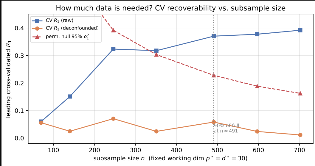
Figure 21: Data-requirement sweep on ADNI at fixed working dimension p^* = d^* = 30 . The raw \hat{R}_1^{\text{cv}} (blue) clears the shrinking permutation null (red) near n \approx 350 and plateaus; the demographic-deconfounded \hat{R}_1^{\text{cv}} (orange) stays flat near zero at every n . More data detects the raw channel but never rescues the deconfounded one.
