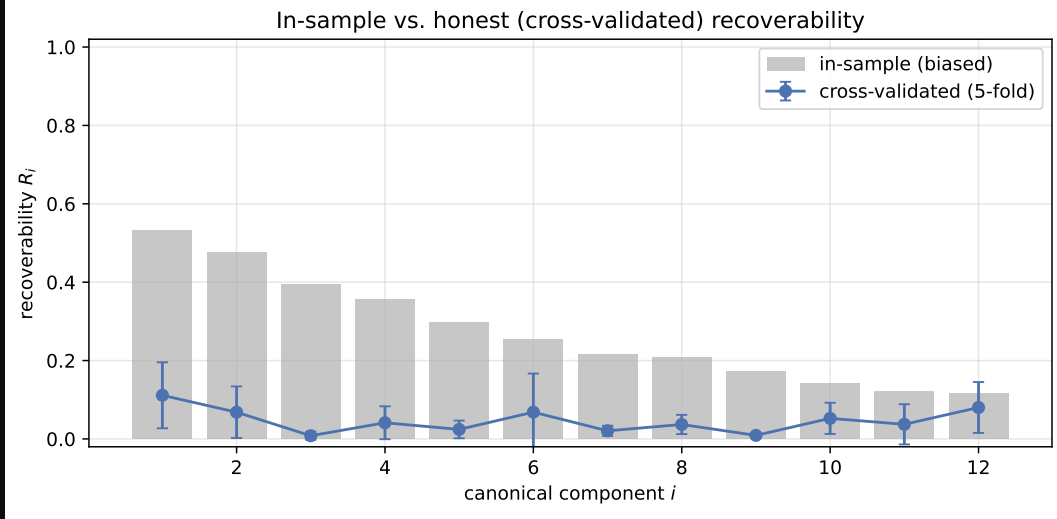
Figure 16: Recoverability spectrum on NSCLC ( n = 129 , organ radiomics, copula marginals). The leading cross-validated \hat{R}_1^{\text{cv}} \approx 0.11 (blue) is only marginally above the permutation null and, unlike at small n , does not generalize: the held-out R^2 of the leading direction is negative and the channel fails de-confounding.
