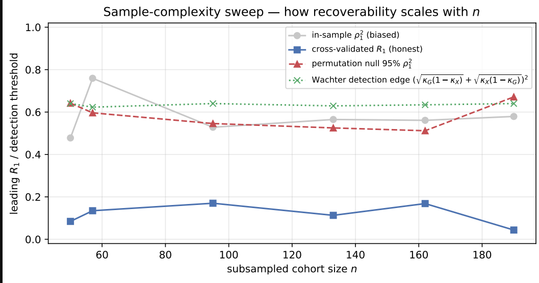
Figure 14: Sample-complexity sweep on TCGA-KIRC. Honest \hat{R}_1^{cv} (blue squares) stays in a low band ( \approx 0.04 – 0.17 ) across cohort sizes without a clear trend; in-sample \hat{\rho}_1^2 (grey) is dominated by the high-dimensional bulk; the permutation 95% null (red triangles) and Wachter edge (green crosses) sit above the honest recoverability at every n .
