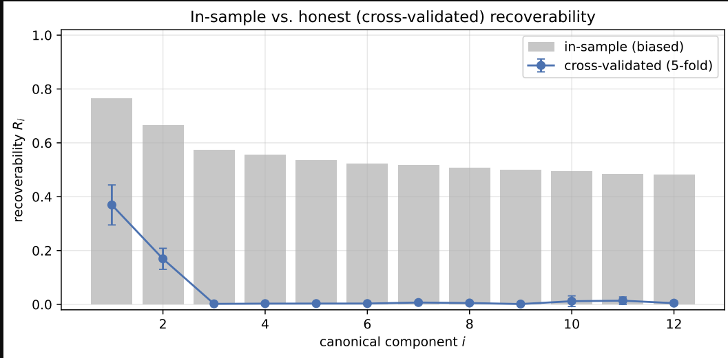
Figure 17: Recoverability spectrum on ADNI ( n = 702 , FastSurfer morphometry + PyRadiomics, copula marginals). The honest cross-validated spectrum (blue) resolves two genomic directions ( \hat{R}_1^{\text{cv}} = 0.37 , \hat{R}_2^{\text{cv}} = 0.17 ) above the permutation null before collapsing — the strongest and highest-rank channel of the three cohorts (compare Figs. 12, 16).
