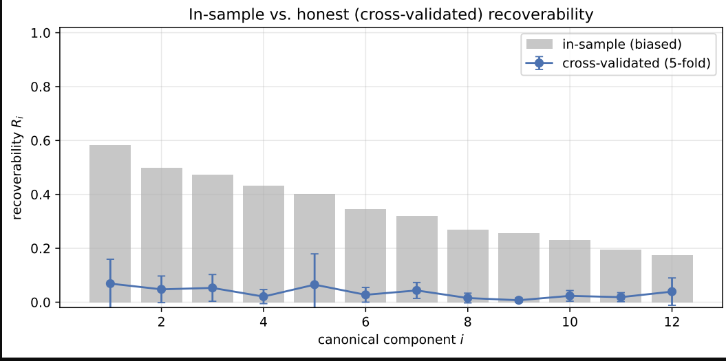
Figure 12: Recoverability spectrum on TCGA-KIRC (organ radiomics, copula marginals). In-sample \hat{R}_i (grey) is biased upward by the high-dimensional geometry; cross-validated \hat{R}_i (blue, 5-fold) is a small positive residual whose leading component is permutation-significant across preprocessing variants. The NSCLC leading direction (Fig. 16) is of similar magnitude but, unlike KIRC’s, does not generalize or survive de-confounding at full n .
