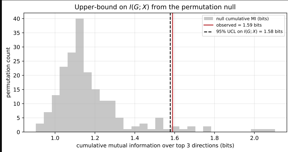
Figure 13: Cumulative-MI null distribution (top-3 canonical components) on TCGA-KIRC. The observed value (red) sits at the upper edge of the null bulk; the dashed line marks the 95% upper confidence limit on I(G; X) used in (26).
