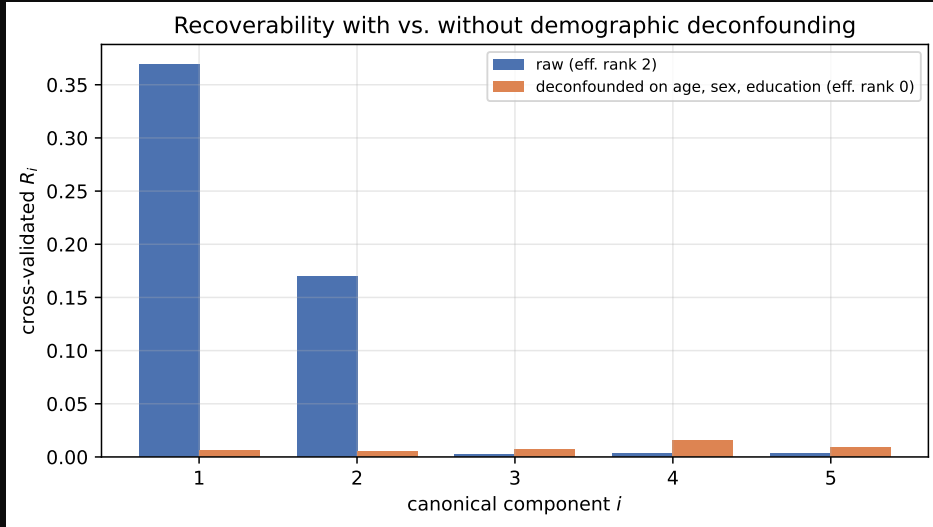
Figure 20: Demographic deconfounding on ADNI. Honest cross-validated recoverability spectrum before (blue) and after (orange) regressing age, sex, and education out of both modalities. The raw rank-two channel ( \hat{R}_1^{cv} = 0.37 ) collapses to a null ( \hat{R}_1^{cv} = 0.006 , \hat{k}_{eff} = 0 , permutation p = 0.48 ): the ADNI association is almost entirely demographically mediated.
