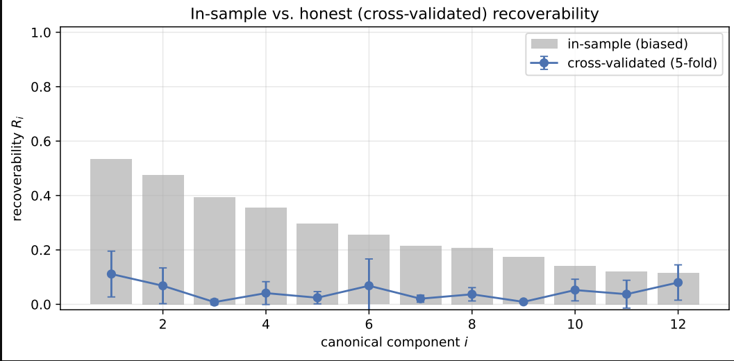
Figure 13: Recoverability spectrum on NSCLC ( n = 129 , organ radiomics, copula marginals). The leading cross-validated \hat{R}_1^{cv} \approx 0.11 (blue) is only marginally above the permutation null and, unlike at small n , does not generalize: the held-out R^2 of the leading direction is negative and the channel fails de-confounding.
