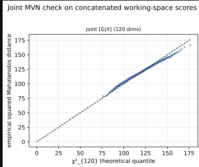
Figure 10: Joint-MVN check on the concatenated working-space scores [G_{\text{pca}}, X_{\text{pca}}] for the synthetic instance: squared Mahalanobis distances against \chi^2_p quantiles lie on the line, with kurtosis ratio \approx 1 and a 0.4% tail beyond the 99% shell. The real cohorts (Fig. 11) depart from this in their upper tails.
