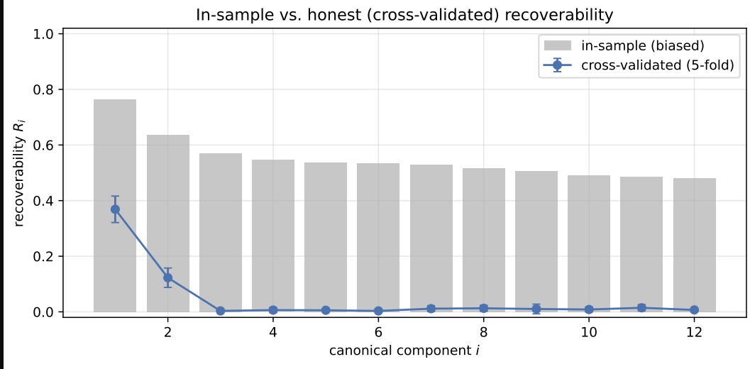
Figure 13: Recoverability spectrum on ADNI ( n = 702 , FastSurfer morphometry + PyRadiomics, copula marginals). The honest cross-validated spectrum (blue) resolves two genomic directions ( \hat{R}_1^{cv} = 0.37 , \hat{R}_2^{cv} = 0.12 ) above the permutation null before collapsing — the strongest and highest-rank channel of the three cohorts (compare Figs. 8, 12).
