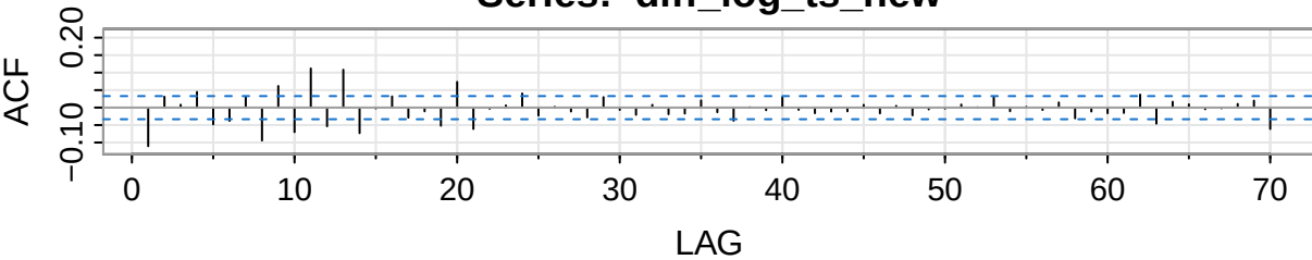
Series: diff_log_ts_new
