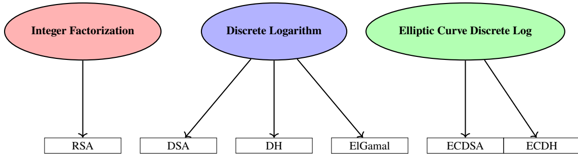
Fig. 3.6 The three computational hardness assumptions and the cryptosystems they support. Every deployed public-key primitive traces its security to one of these three problems.
